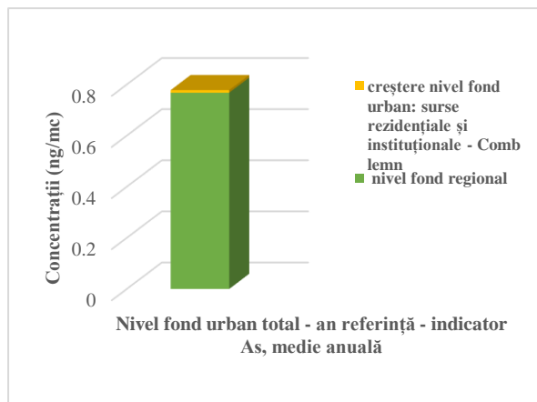
Figura nr. 3-93 Nivel Fond urban total – indicator As
